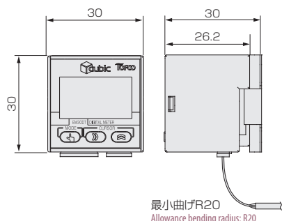
EM30DT EM30DT outside deminsional drawing
