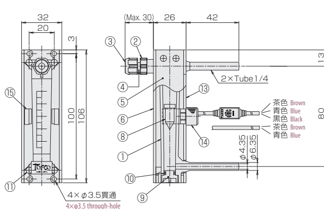
PF200/300 光電センサ付 with photosensor
