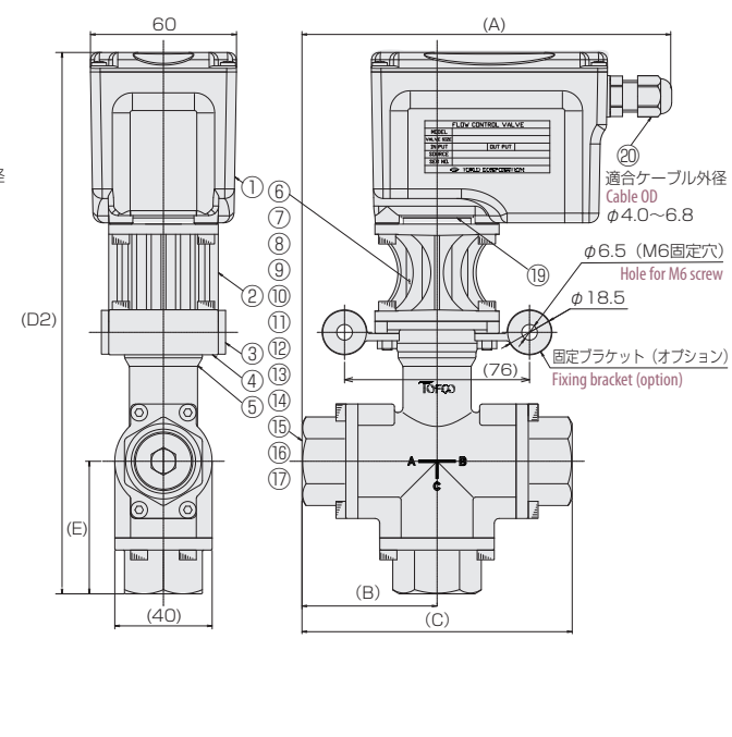
FCV-NH32T 3方弁 3-way valve
