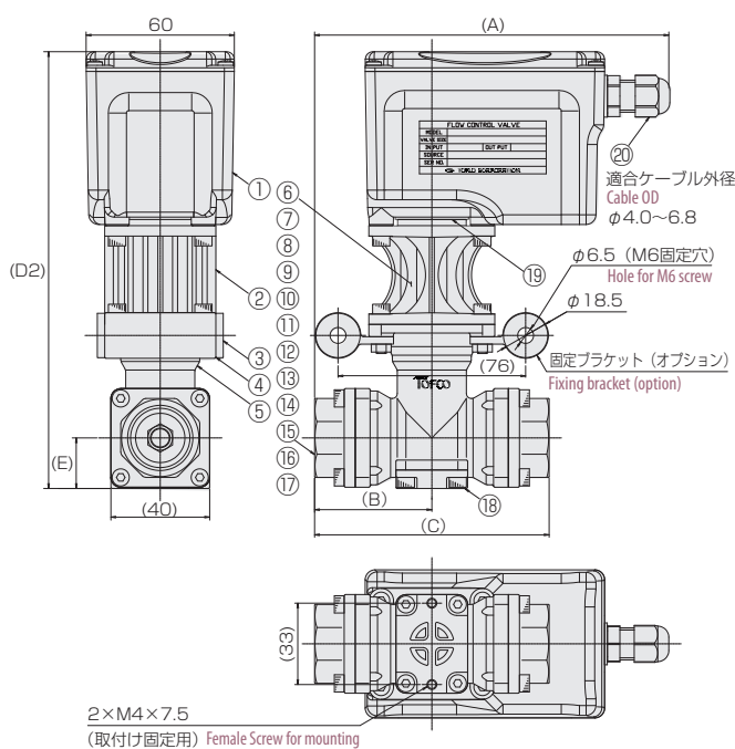
FCV-NH□S 2方弁 2-way valve
