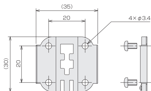
取付板 Mounting adapter
