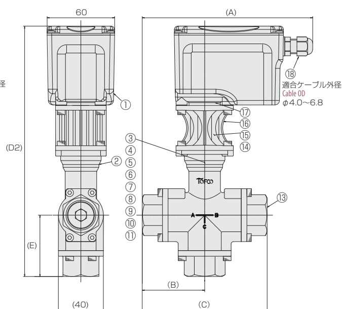
FCV-NH32T 3方弁 3-way valve
