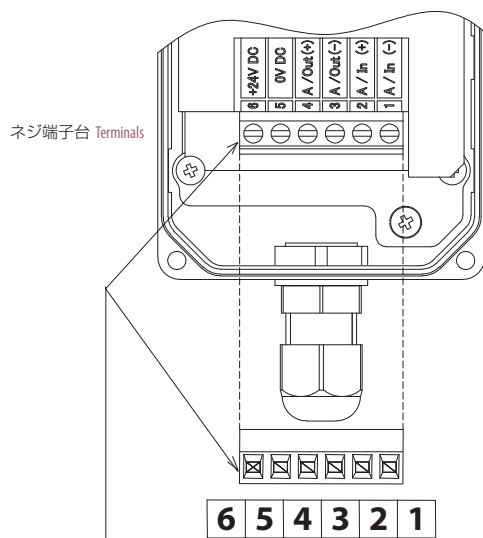
ピンNo. Pin No. for Terminals
