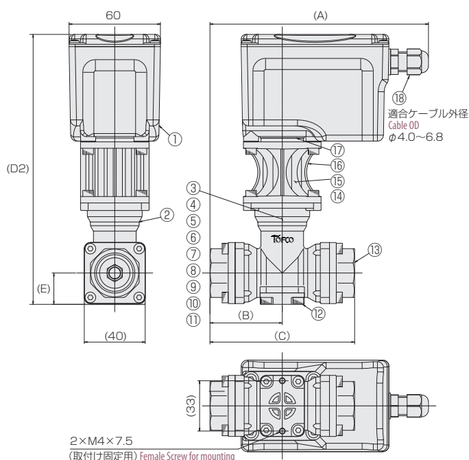
FCV-NH□S 2方弁 2-way valve
