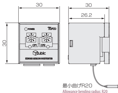
EX30AR EX30AR outside dimensional drawing
