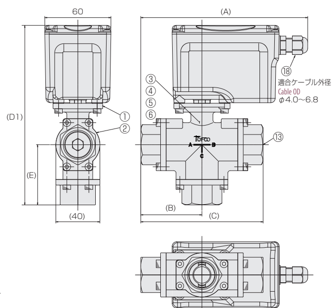
FCV-N32T 3方弁 3-way valve
